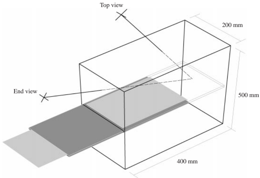
FIGURE 1. Sketch of experimental apparatus. The hollow stainless steel barrier is shown as dark grey and the nylon fabric as light grey. The orientation of the perspective views presented in §4.2 are also indicated.
